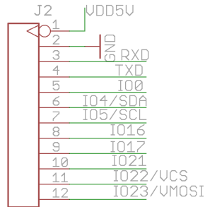
HEADER-12P-2.54
